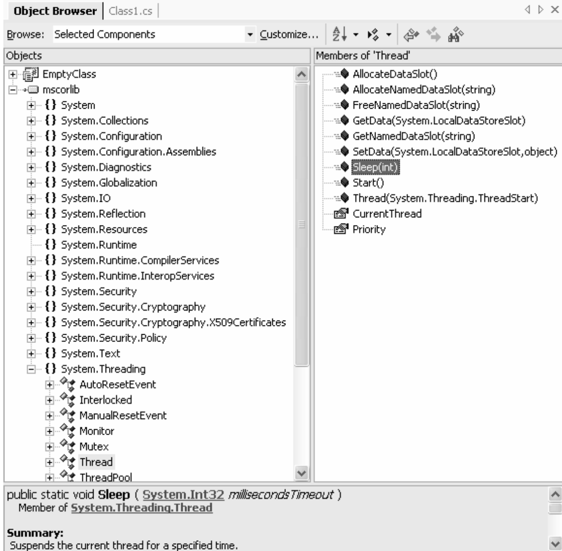
Figure 3-3 The Object Browser showing the contents of mscorlib.dll [Comment 3.36]
